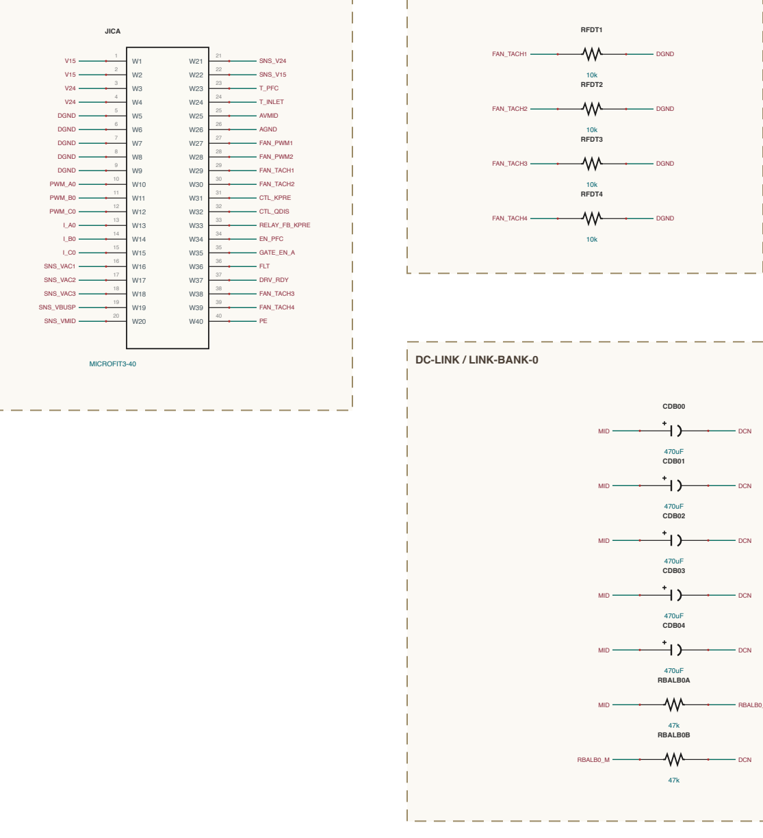
AUX-POWER / INTERCONNECT
