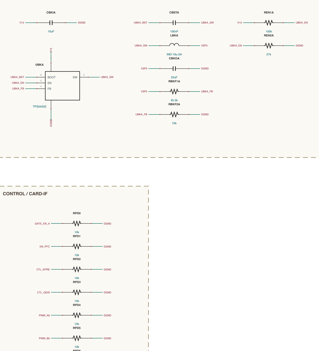
AUX-POWER / BUCK-DVD
