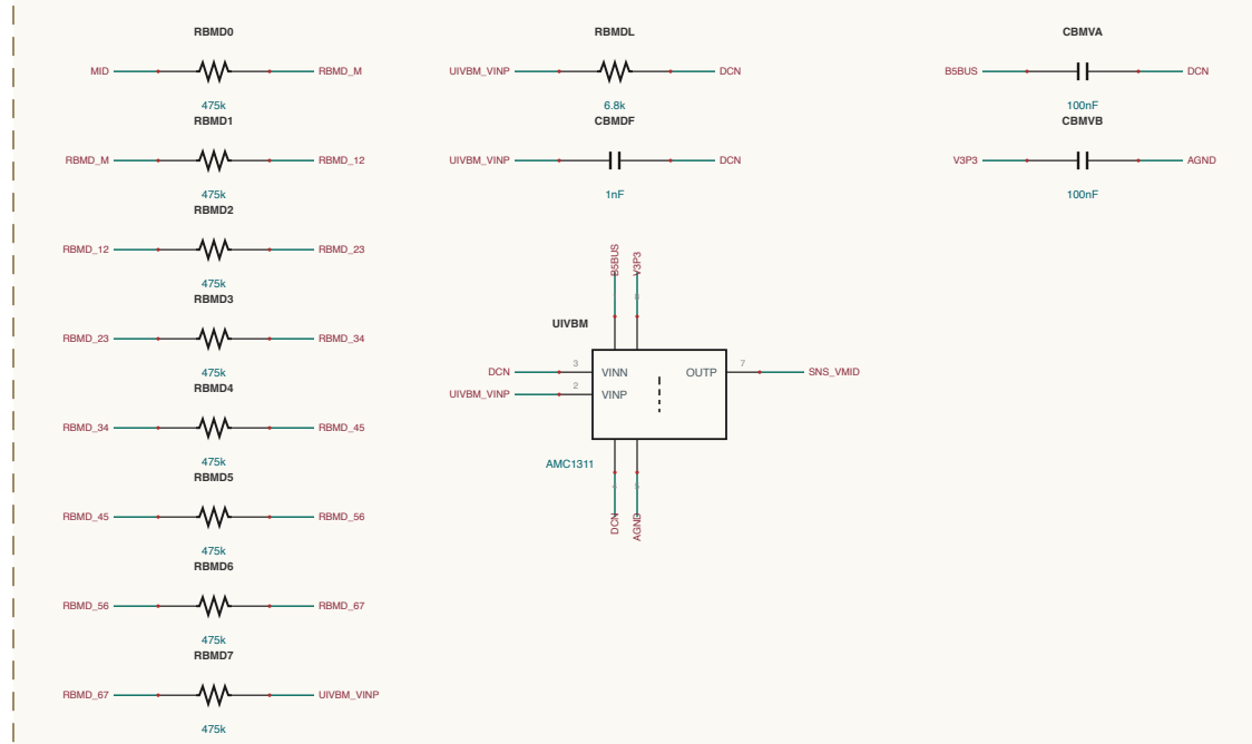
AC-SENSING / SENSE-VMD
