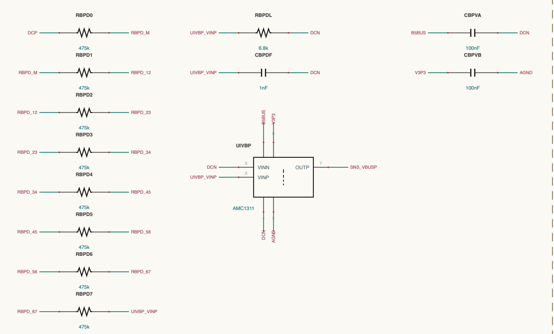
AC-SENSING / SENSE-VIBUS
