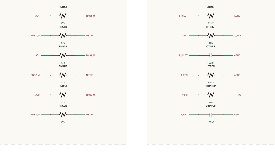
AUX-POWER / INTERCONNECT
