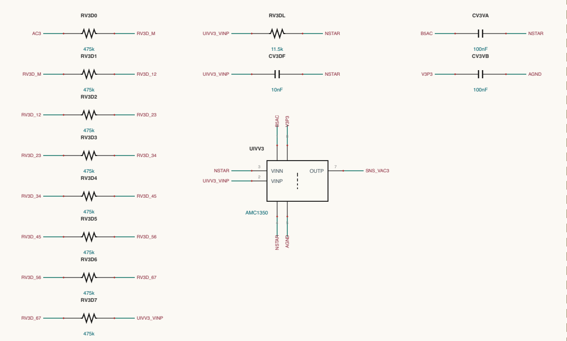
AC-SENSING / SENSE-VAC3
