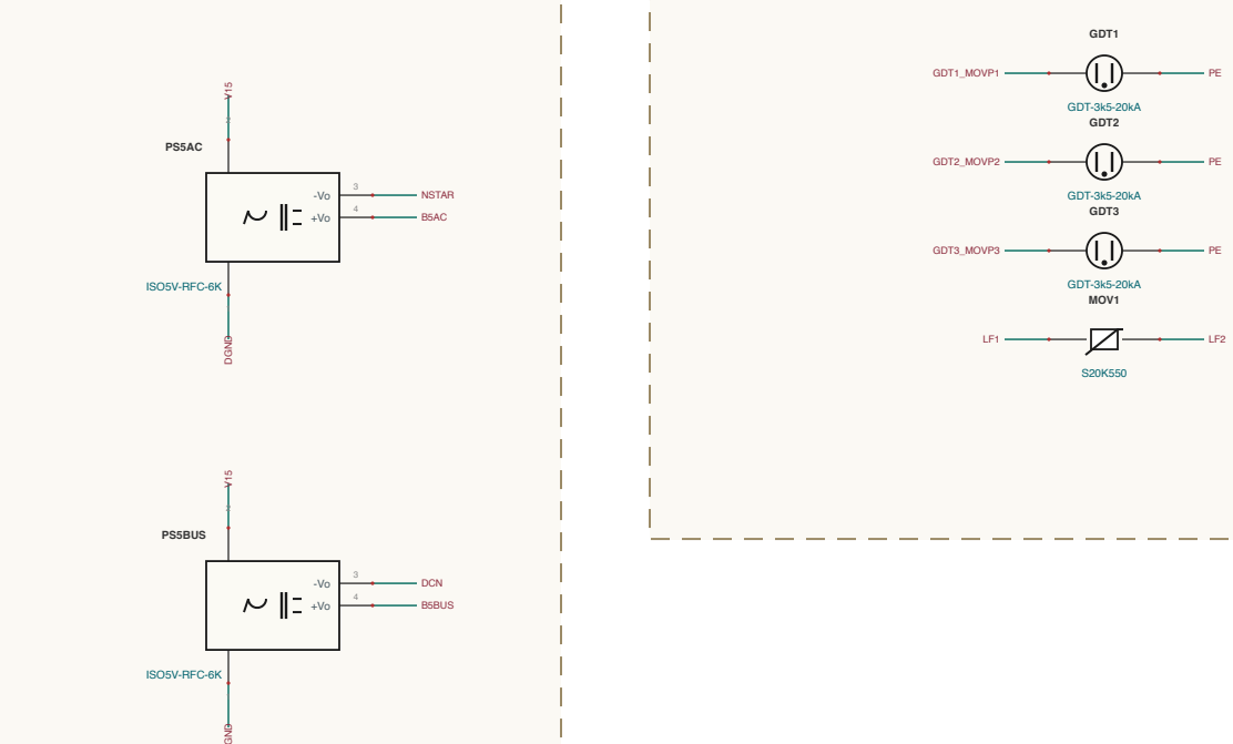
AC-SENSING / ISO-BIAS
