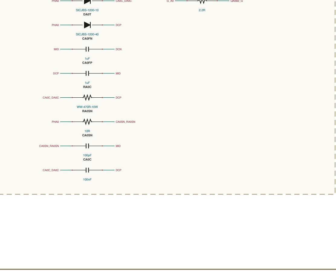
DC-LINK / LINK-BANK-10
