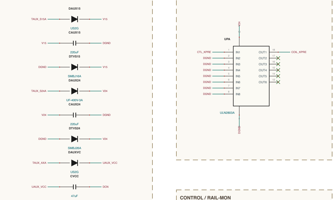
AUX-POWER / FANS
