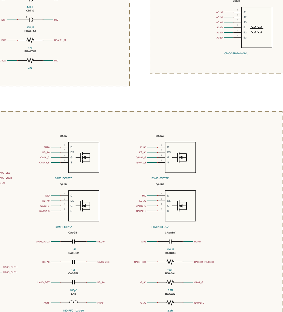
DC-LINK / LINK-BANK-10
