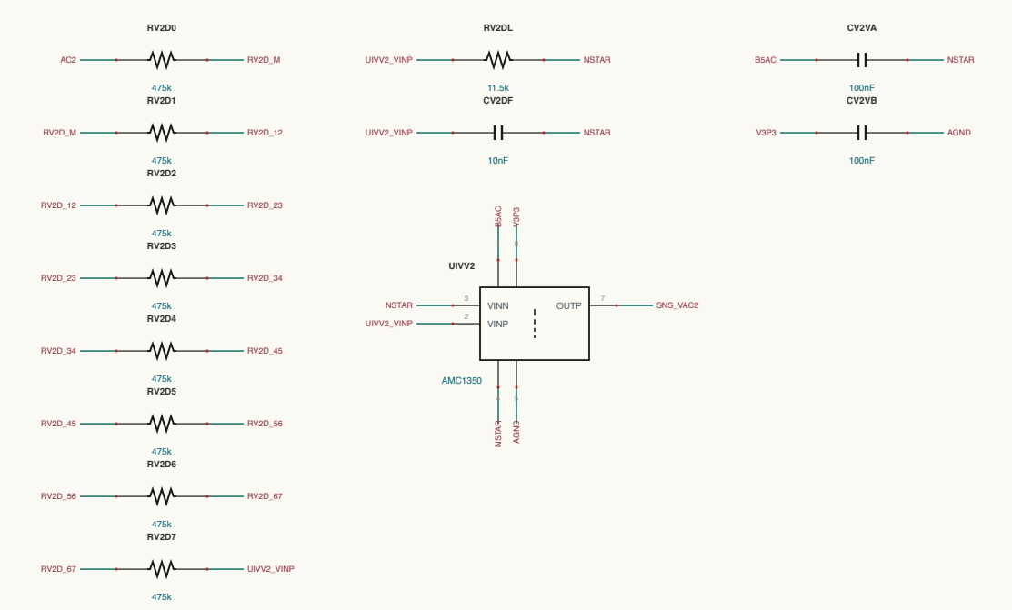
AC-SENSING / SENSE-VAC2
